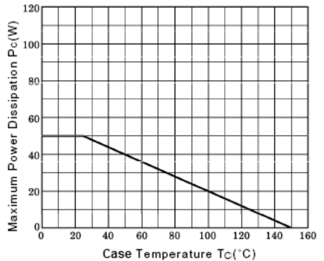
Power Derating
